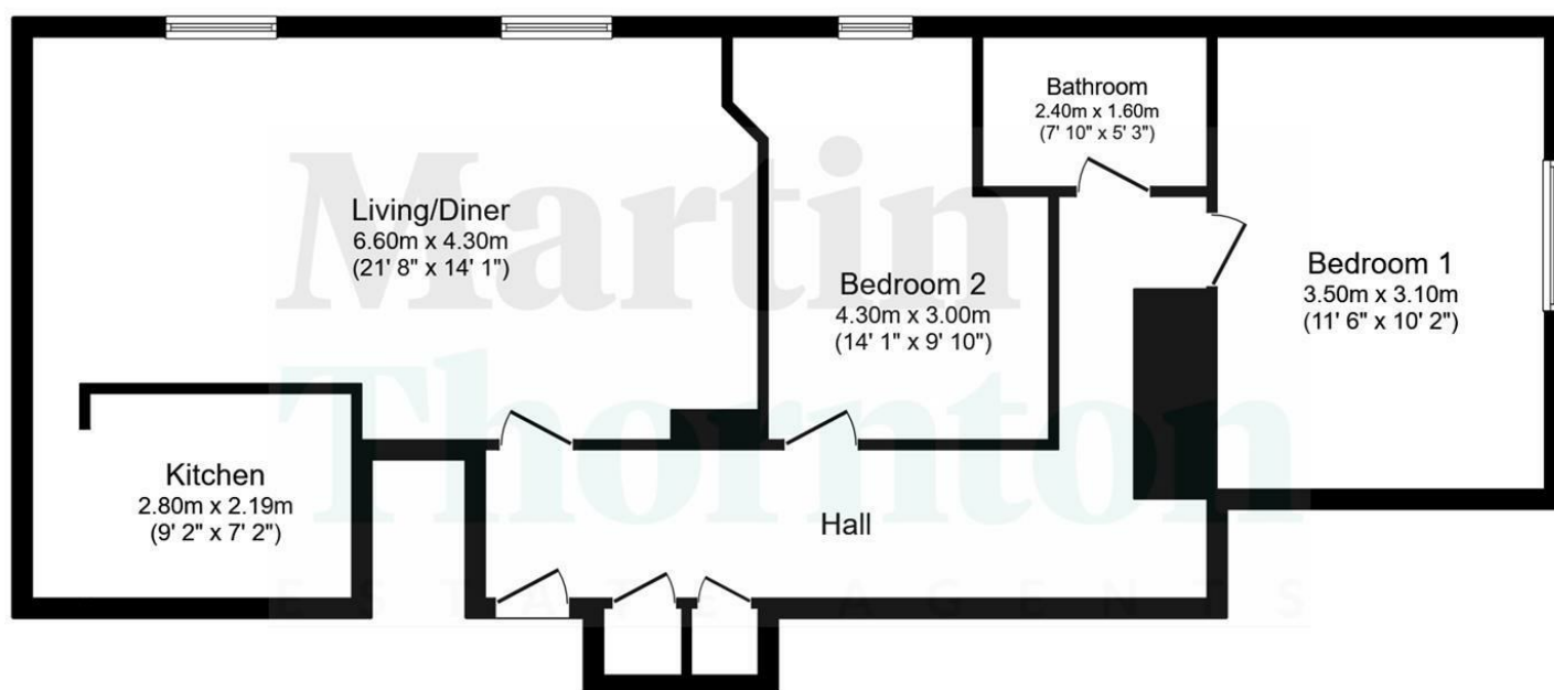
Floor Plan
